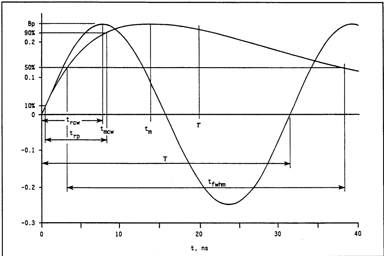
Figure 1. Relationship between exponential pulse and sine wave.
