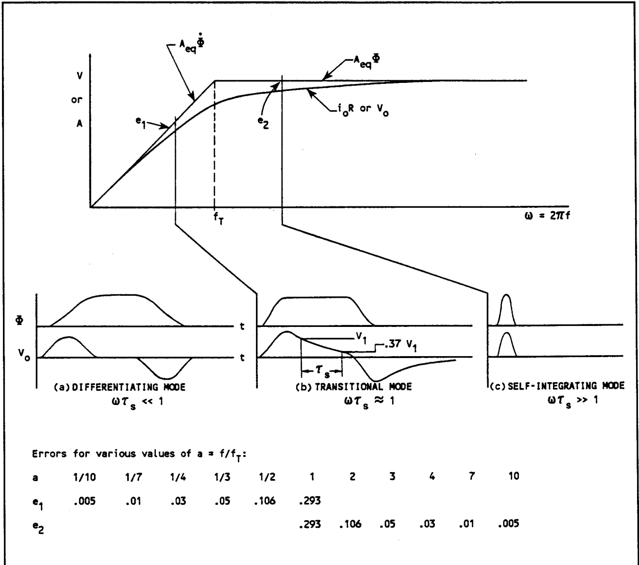
Figure 3. Operating modes of field sensors.
