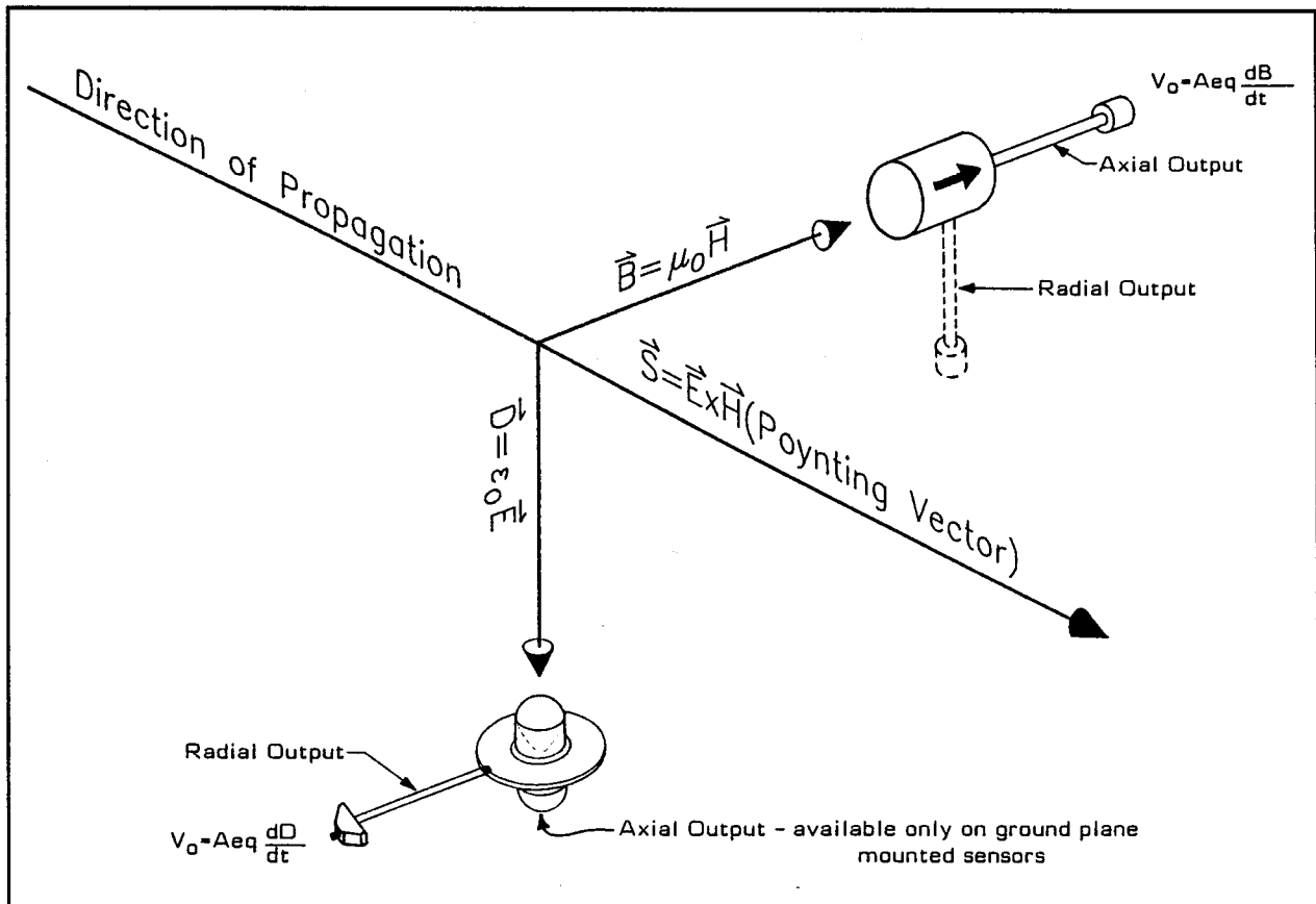
Figure 2. Electric and magnetic fields being measured with D-dot and B-dot sensors.
