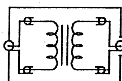
3. Grounded Unbalanced Floating Unbalanced (GUFU)
