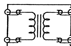
4. Grounded Balanced Floating Balanced (GBFB)
